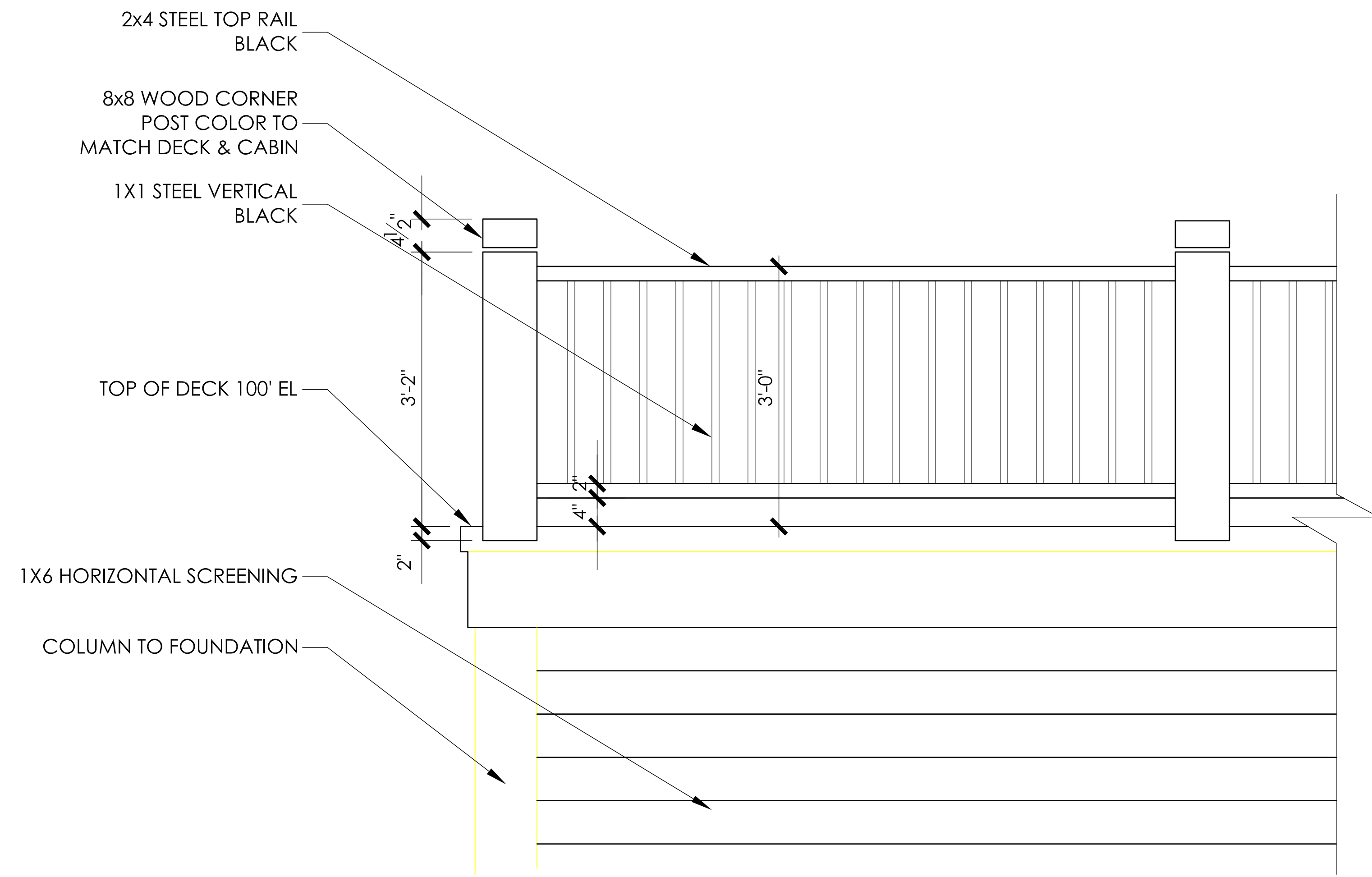
2 A3.2 DECK RAILING DETAILS SCALE: 1/2" = 1'-0"
